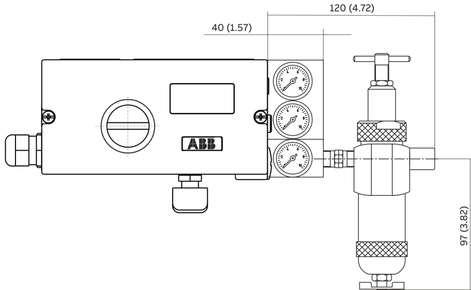
Figure 20: Positioner DS_TZIDC_EN_G with mounted pressure gauge block and filter regulator
